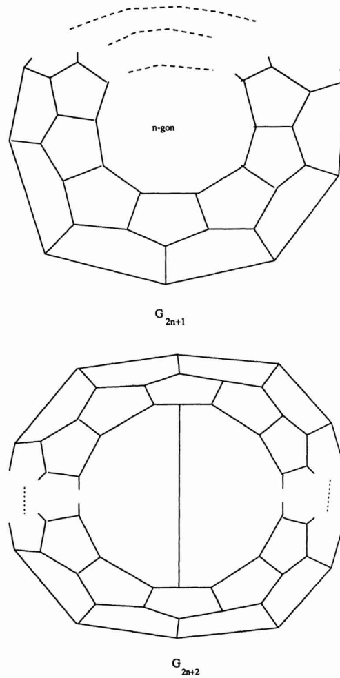
Fig. 1. The graphs G_g
