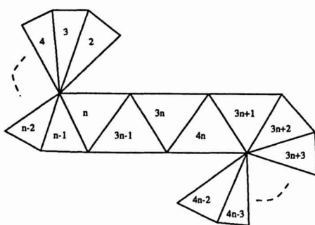
B subset, odd genus case g = 2n+1
