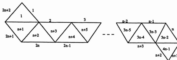
A subset, odd genus case g = 2n+1
