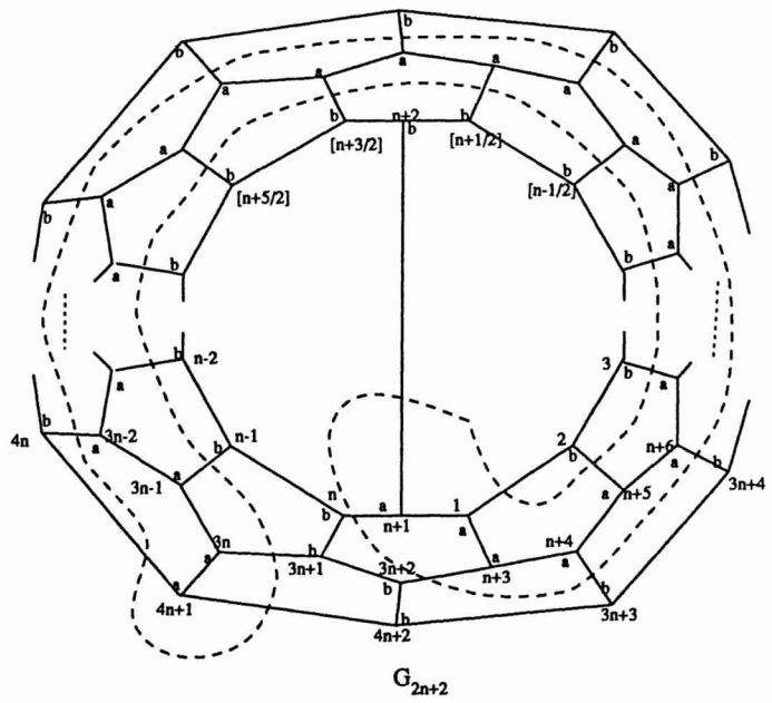
Fig. 2. The labelled graphs G_g
