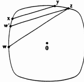
Fig. 2.2. Comparing chords \mathbf{wz} and \mathbf{xy} .
