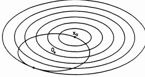
Fig. 2.6. (t \partial B + x_0) \cap \partial B for 0 \leq t \leq 2 .
