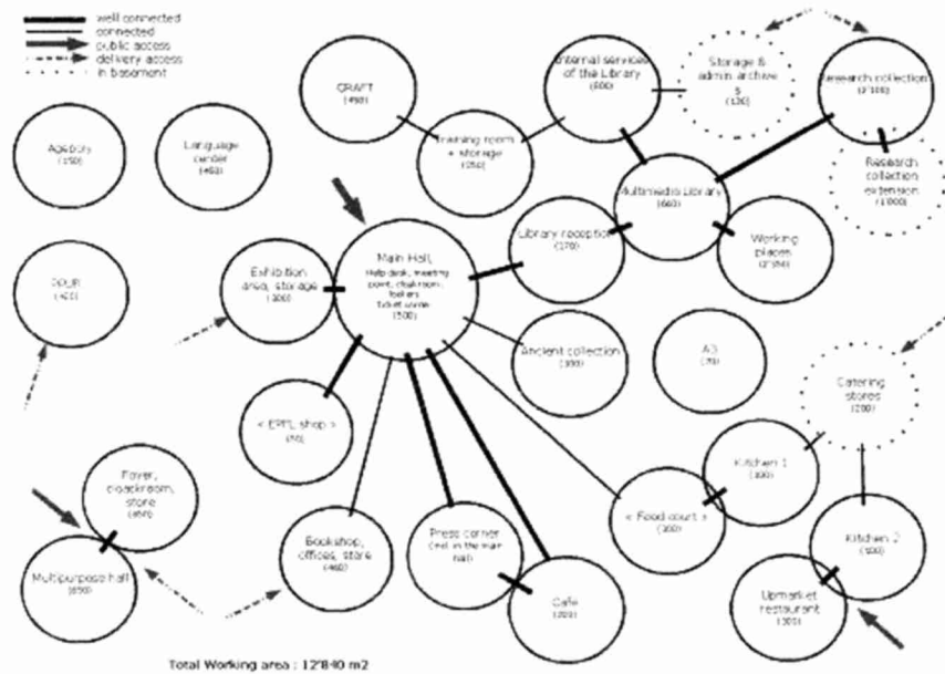
Fig. 10: Functional layout of Learning Center
